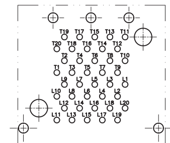
CONNETTON PINOUT DETAIL COMPONENT SIDE OF BOARD
